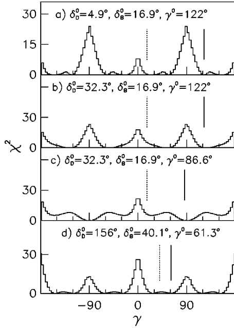
FIG. 1. \chi^2(\xi) as a function of \gamma for different values of the actual phases, \delta_D^0 , \delta_B^0 , \gamma^0 . For each value of \gamma , \chi^2(\xi) is minimized with respect to B(B^+ \rightarrow D^0 K^+) , \delta_D and \delta_B . The points \gamma = \gamma^0 and \gamma = \delta_B^0 are shown by a solid and a dotted line, respectively. Some asymmetry and noise are due to the dependence of the fit on the initial \xi values. (a) The 8-fold ambiguity of Eqs. (4) and (6) is demonstrated for small \delta_D^0 . (b) Increasing \delta_D , the S_{\text{exchange}} ambiguity is resolved. (c) With \gamma close to 90^\circ , the S_\pi and S_{\text{sign}} ambiguities overlap. (d) The S_{\text{exchange}} ambiguity is resolved, but an accidental ambiguity shows up at \gamma \approx 28^\circ , with B(B^+ \rightarrow D^0 K^+) at approximately 4/3 its input value.
